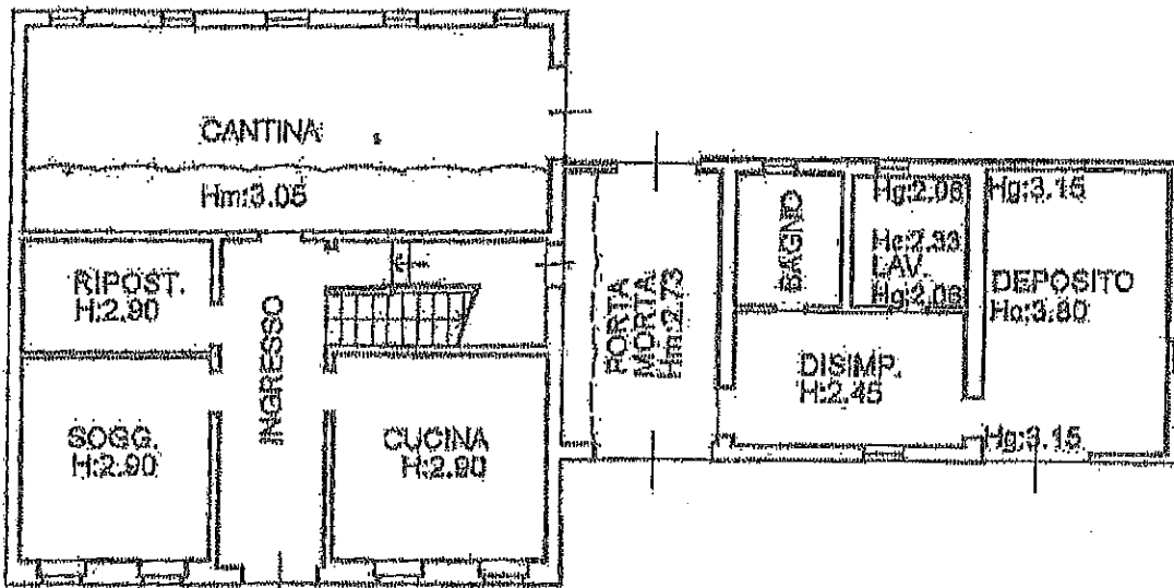
PIANO TERRA
